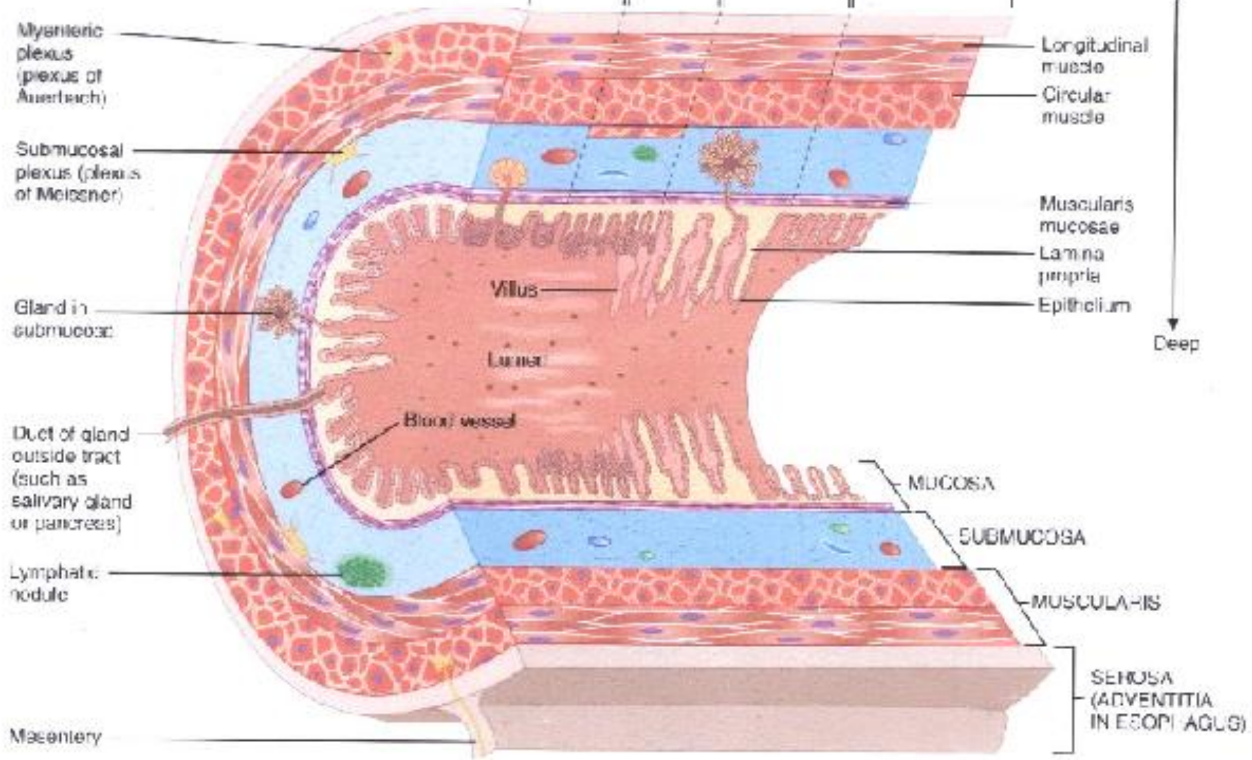
Sectional views of layers of the GI tract
